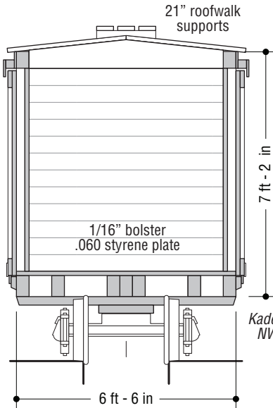
Section at Bolster
