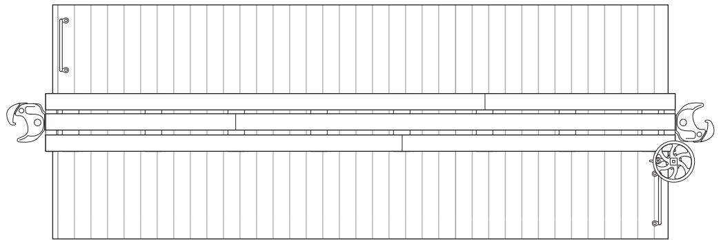
Roof Plan
