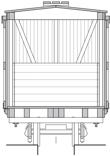
Section at Queen Posts
