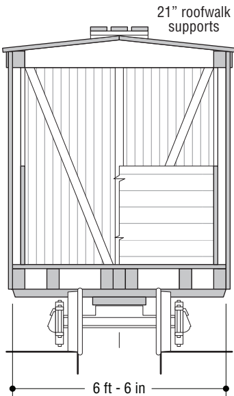
Section at Bolster
