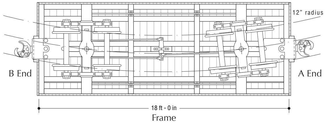
San Juan Evolution Couplers w/ Kadee #807 pockets
