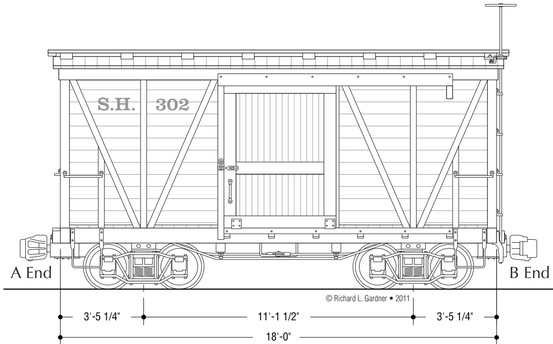
Side Elevation (other side similar)
