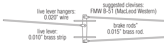
Brake Lever Plan
